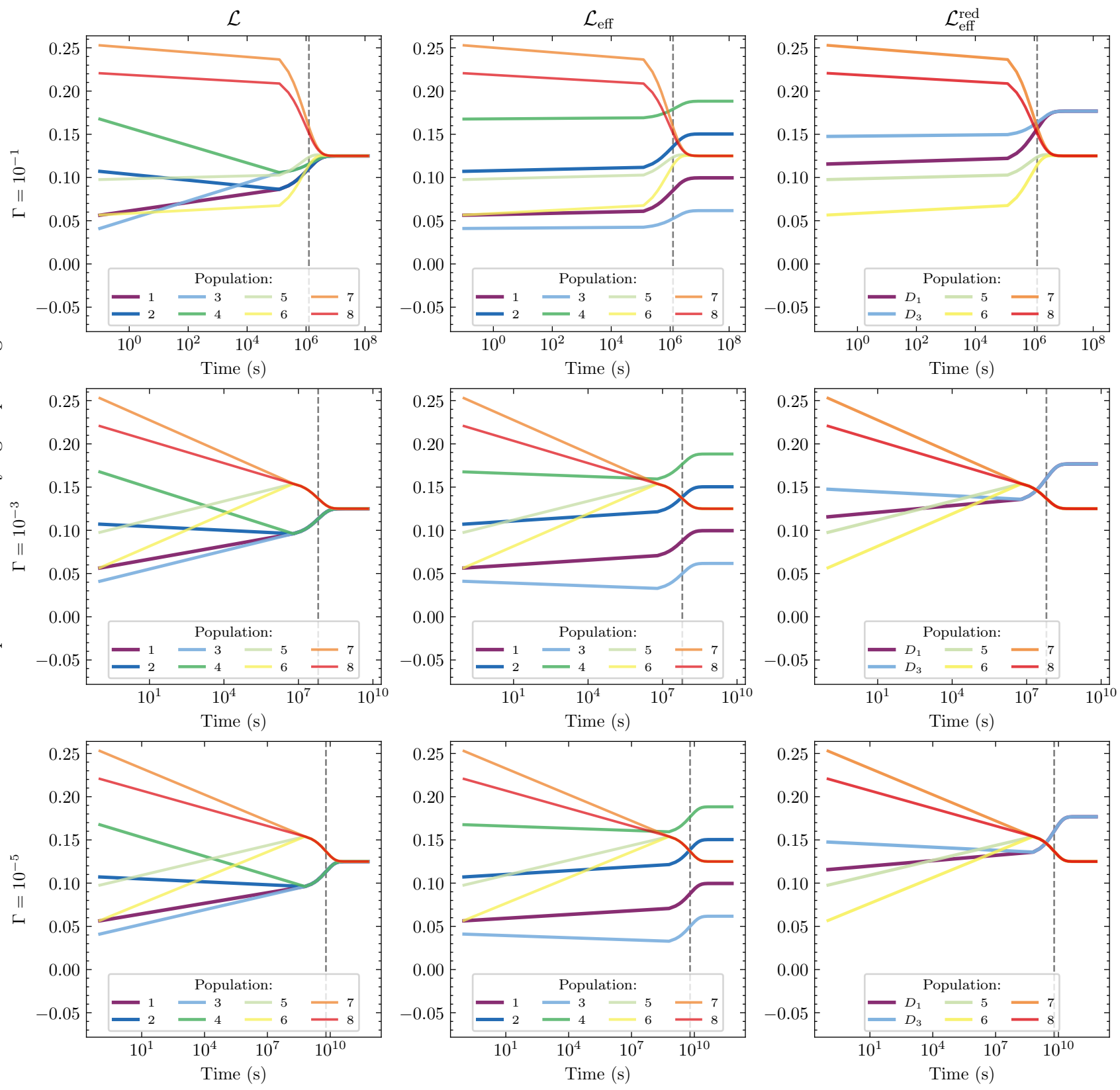
Time Evolution of Site Populations under \mathcal{L} , \mathcal{L}_{\text{eff}} , and \mathcal{L}_{\text{eff}}^{\text{red}} n_d=2 ; n_\epsilon=4 ; J = 10^{-1} ; \epsilon = 10^{-4}
